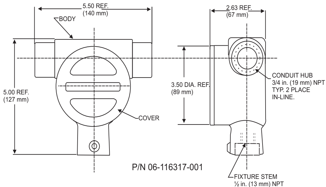
Figure 1. Explosion Proof Junction Box
