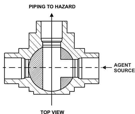
Figure 2. L Flow Ball Position
