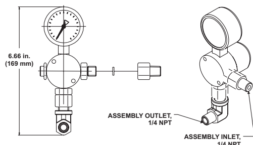
Figure 7. Pressure Regulator
