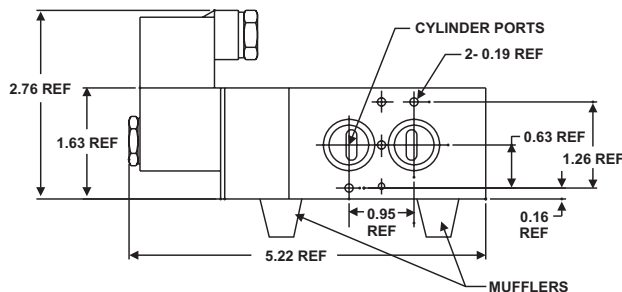
Figure 6. Pneumatic Solenoid
