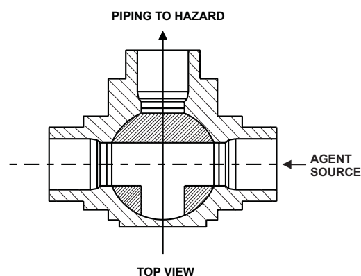
Figure 1. T Flow Ball Position
