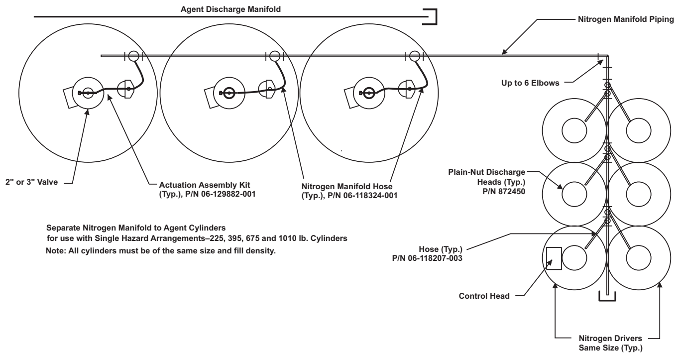
Figure 2. Nitrogen Manifold
