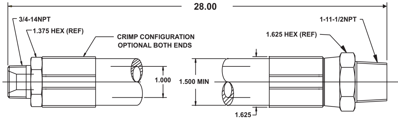
Figure 1. Nitrogen Transfer Hose
