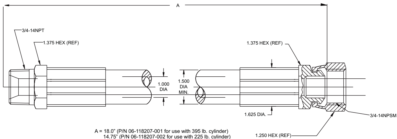
Figure 1. Nitrogen Transfer Hose
