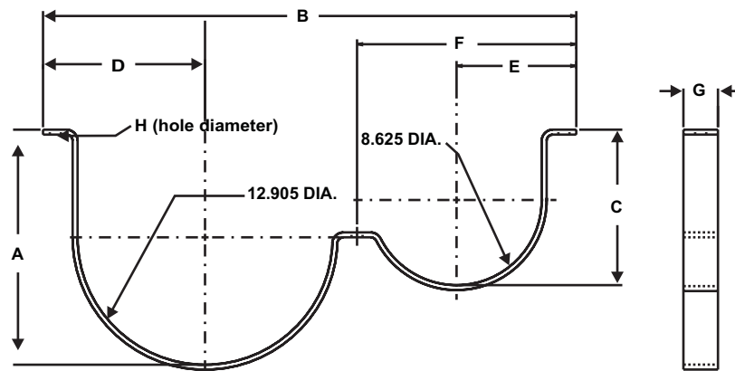
Figure 1. Dimensions for 225 lb. System (P/N 06-236127-001, See Table 1)
