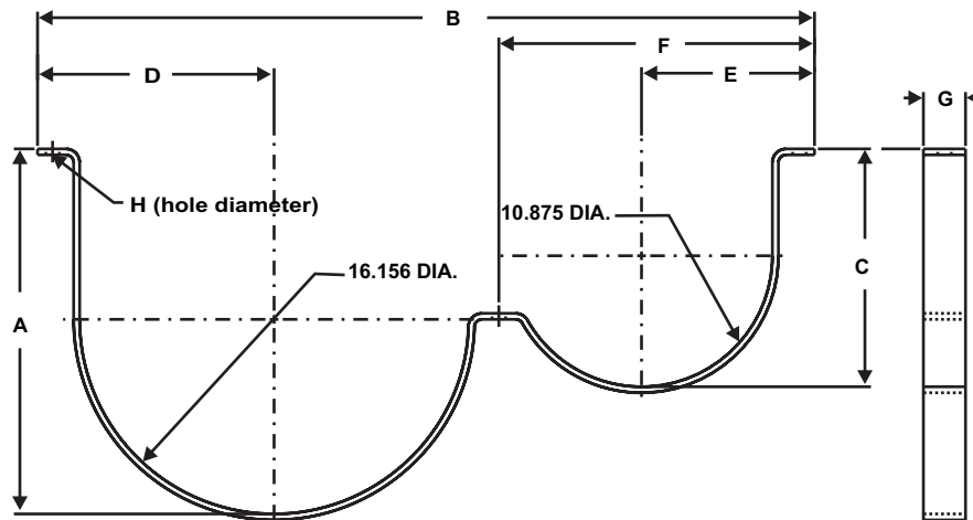
Figure 2. Dimensions for 395 lb. System (P/N 06-236126-001, See Table 1)
