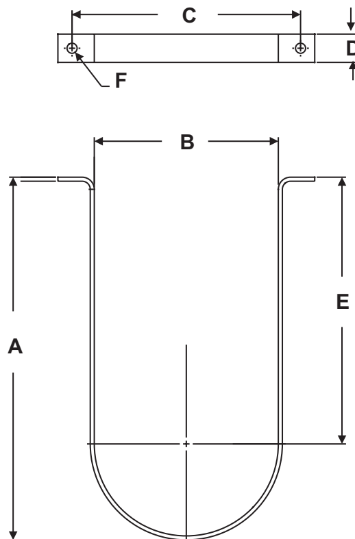
Figure 2. 4890 cu. in. Combined Cylinder Strap (P/N 06-236174-001)
