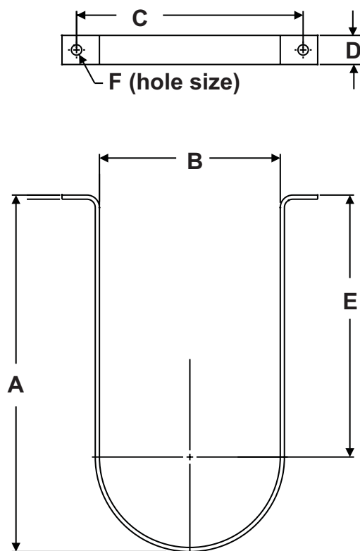
Figure 1. 4070 cu. in. Combined Cylinder Strap (P/N 06-236173-001)
