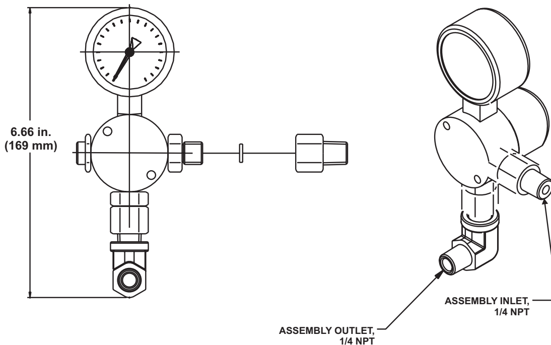
Figure 1. Pressure Relief Dimensions
