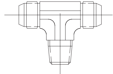
MALE BRANCH TEE 1/8" NPT X 5/16" TUBING P/N 6992-0505
