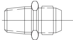
MALE CONNECTOR 1/8" NPT X 5/16" TUBING P/N 6992-0501
