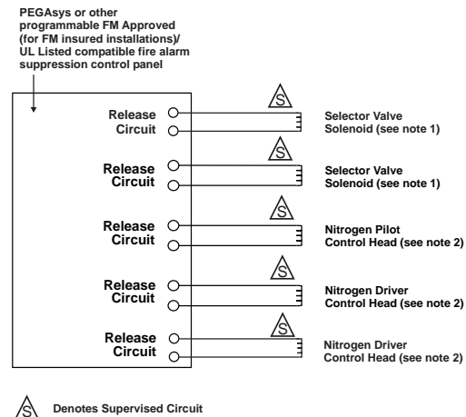
Figure 9. Typical Single Panel System Release Circuit Wiring (see notes below)
