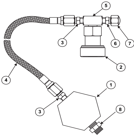
Actuation Kit Assembly
