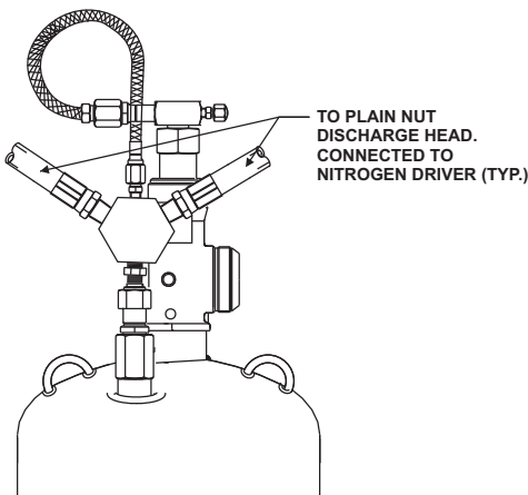
Cylinder and Valve Assembly with Assembled Actuation Components
