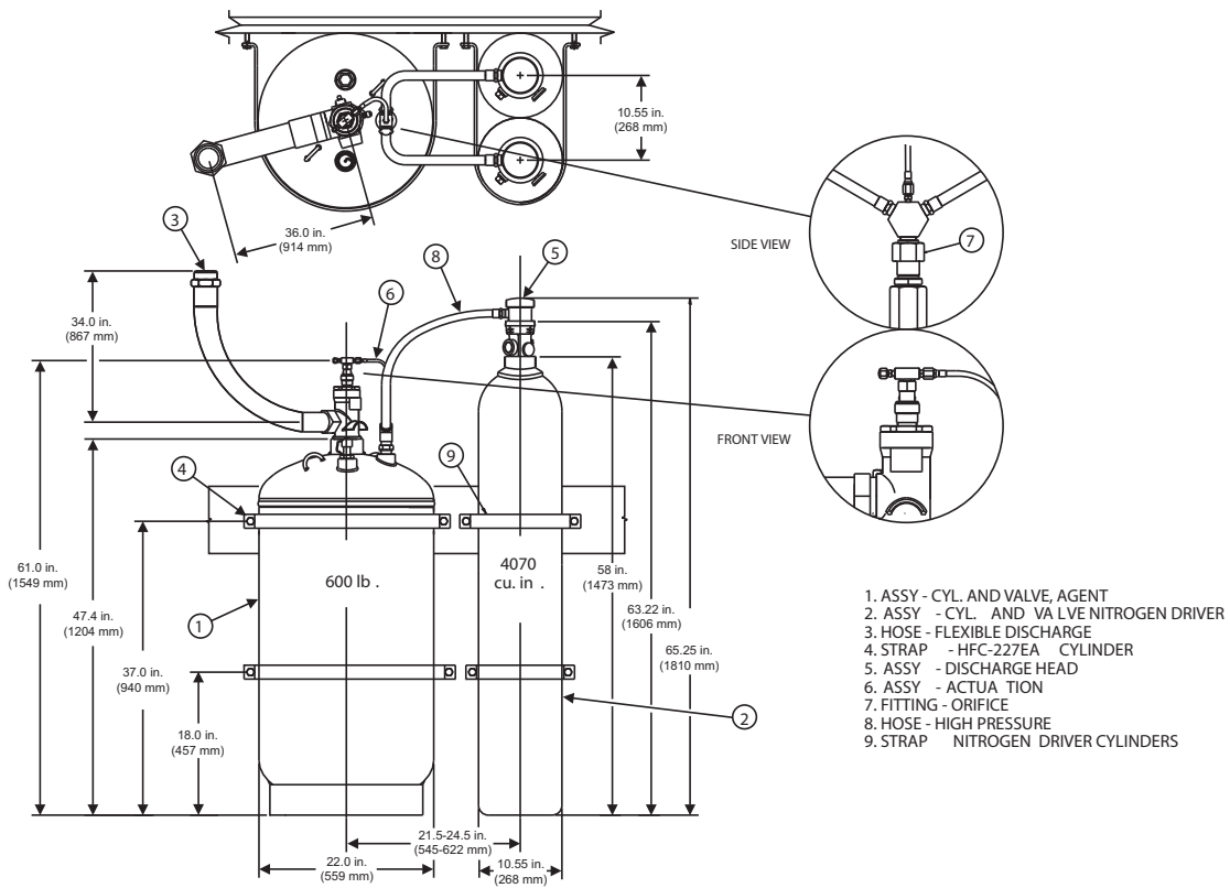
Figure 2. Dual Driver Installation, Vertical Mounting for 600 lb. Systems
