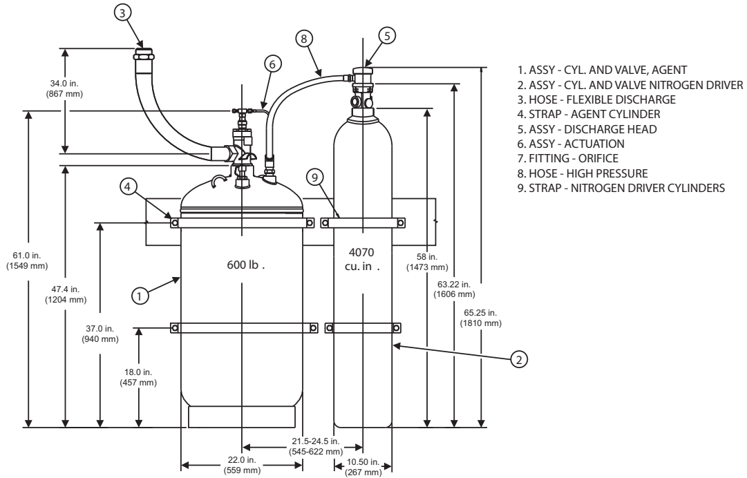
Figure 1. Single Cylinder Installation Dimensions, 600 lb. Cylinder
